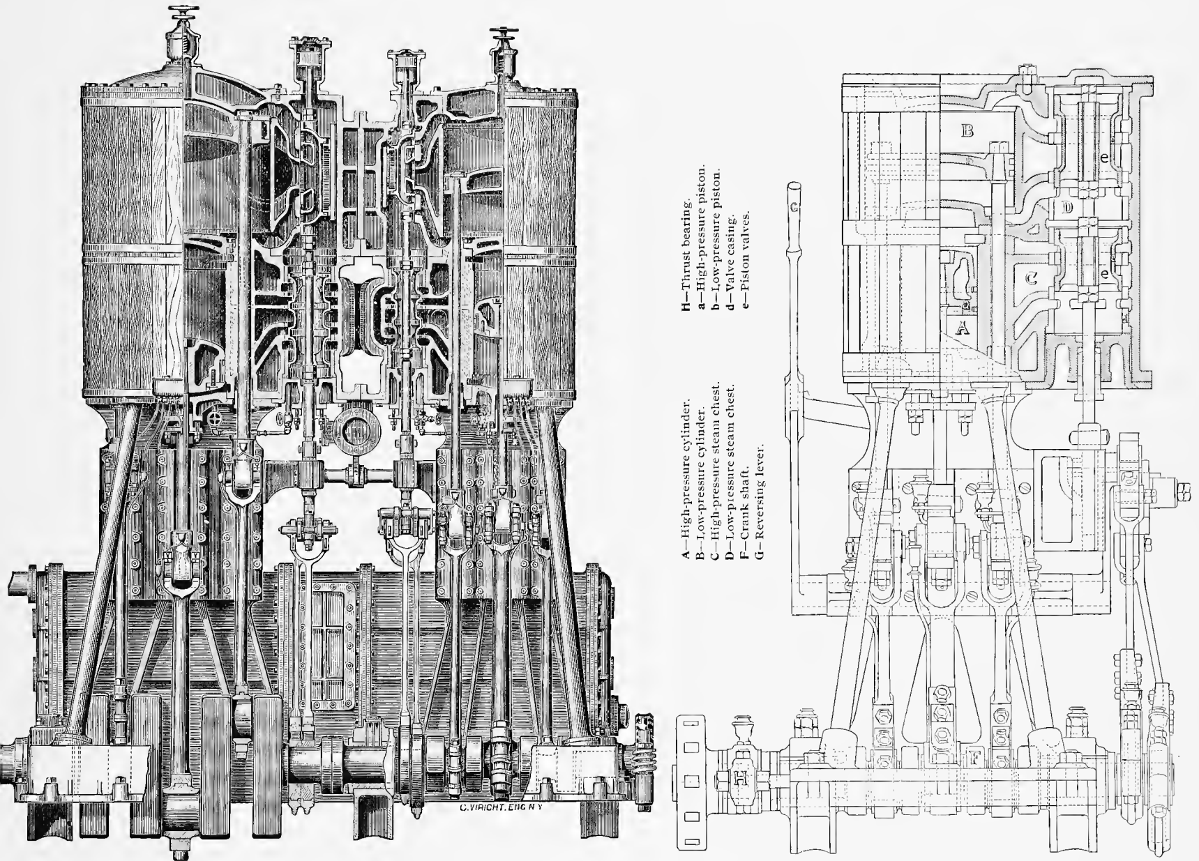
WELLS' PATENT QUADRUPLE-EXPANSION ENGINE.
